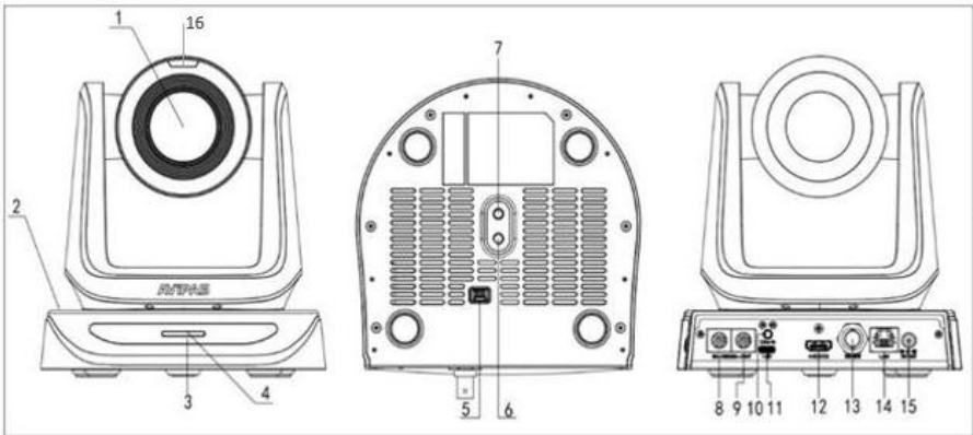
Figure 1.1 Interface Diagram
